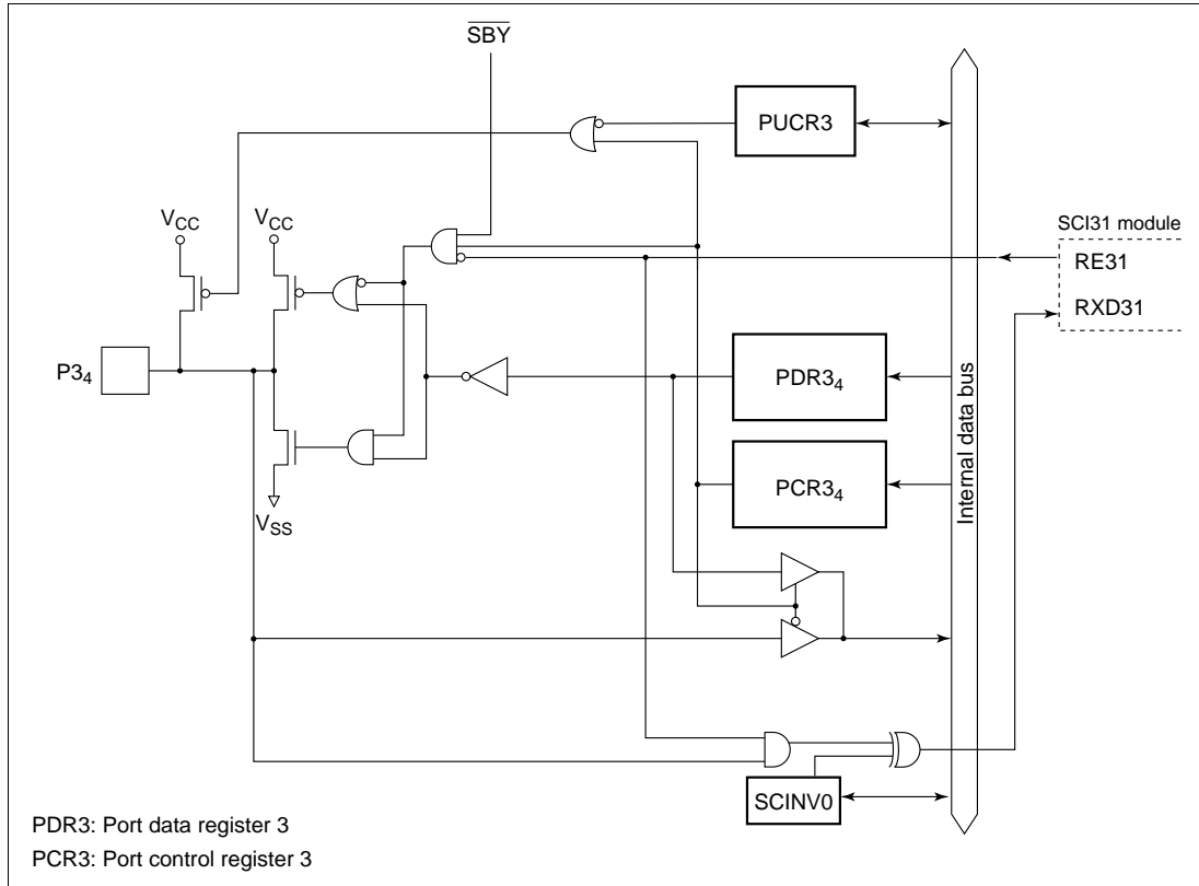
Figure C.2 (c) Port 3 Block Diagram (Pin P34)
