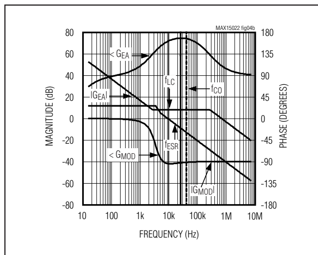
Figure 4b. Power Modulator and Type II Compensator Gain and Phase Response with Lossy Bulk Output Capacitor(s) (Aluminum)
