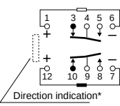
Schematic (Bottom view) 2 coil latching (Reset condition)
