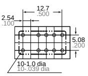
PC board pattern (Copper side view)
