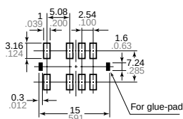
Suggested mounting pad (Top view)
