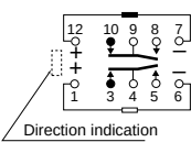
Schematic (Top view) 1 coil latching (Reset condition)
