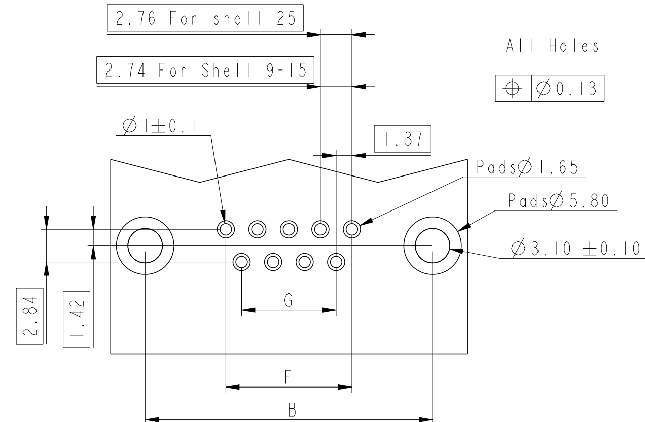
DETAIL A SCALE 8:1
