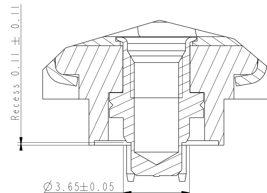
DETAIL A SCALE 8:1
