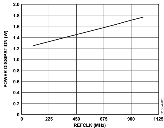
Figure 27. Power Dissipation vs. REFCLK (Single-Tone Mode, f_{OUT} = \text{REFCLK}/5 )
