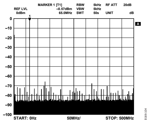
Figure 4. Wideband SFDR, 65 MHz f_{OUT}
