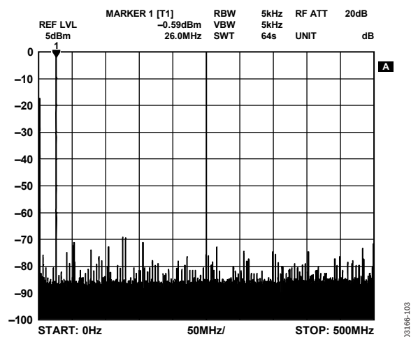
Figure 3. Wideband SFDR, 26 MHz f_{OUT}
