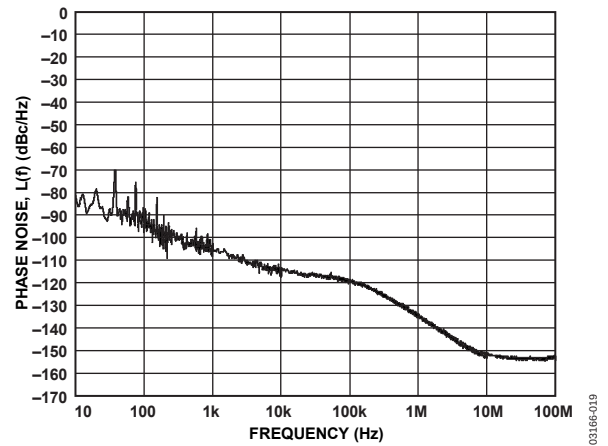
Figure 19. Translation Loop Residual Phase Noise, f_{LO} = 1500 MHz, f_{OUT} = 1550 MHz, Loop BW = 50 kHz
