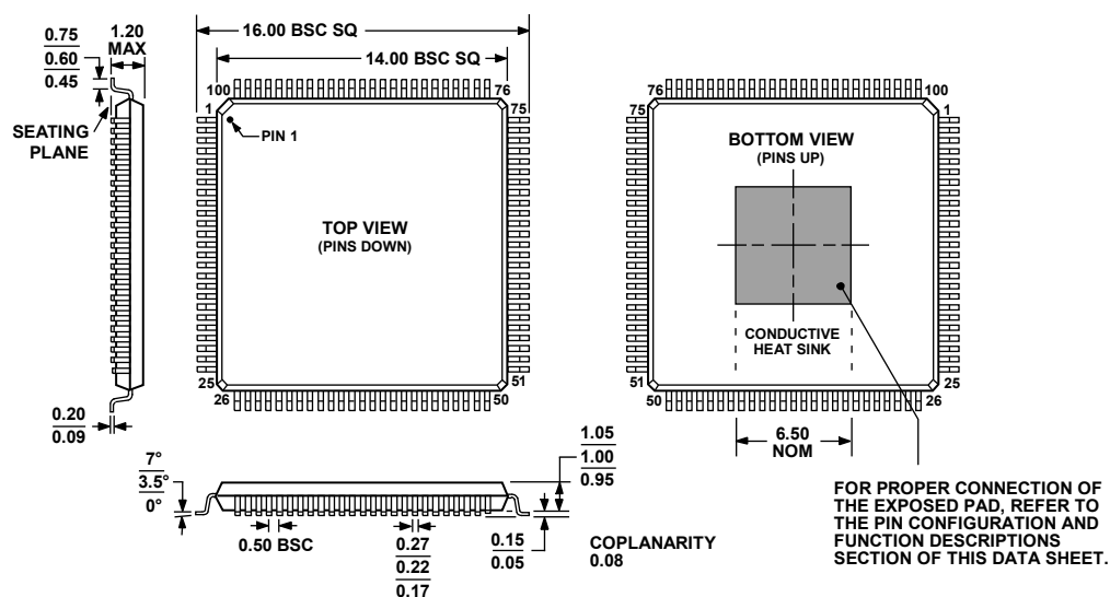
Figure 40. 100-Lead Thin Quad Flat Package, Exposed Pad [TQFP_EP] (SV-100-1)
