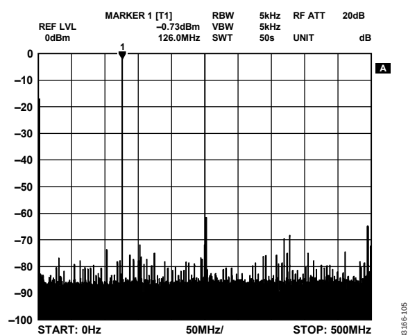
Figure 5. Wideband SFDR, 126 MHz f_{OUT}
