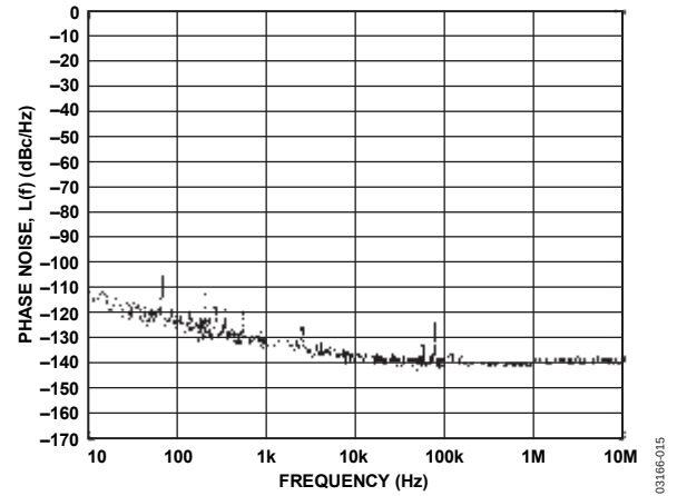
Figure 18. Residual Phase Noise, 403 MHz f_{OUT} , 1 GHz REFCLK
