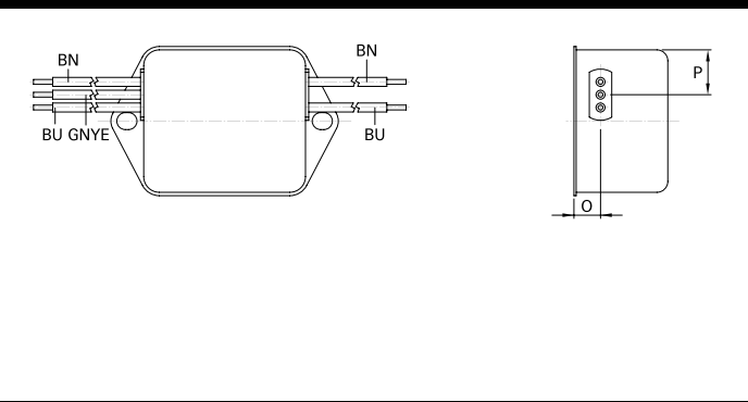
Connection style -07, 1 and 3 A types (same dimensions as style -06)
