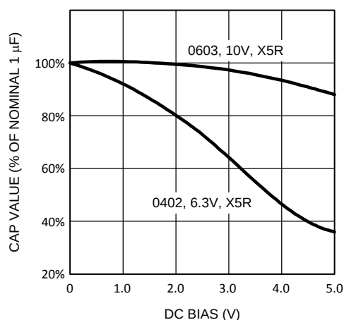
Figure 69. Graph Showing a Typical Variation in Capacitance vs. DC Bias
