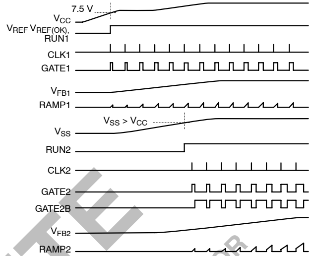
Figure 3. Startup Waveforms
