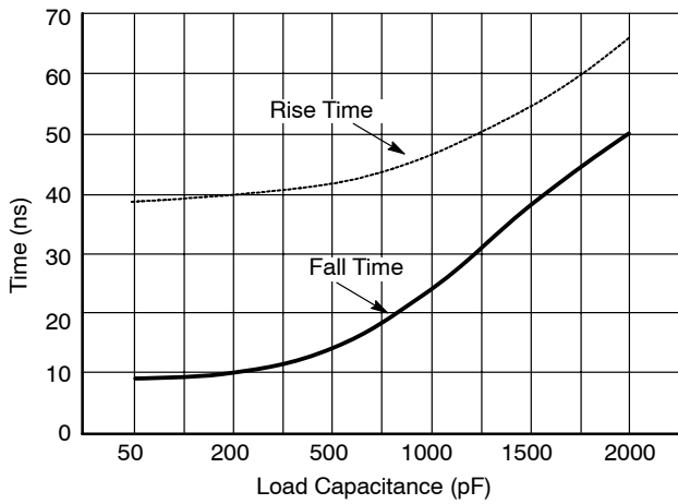
Figure 8. Typical GATE2, 2B Switching Times
