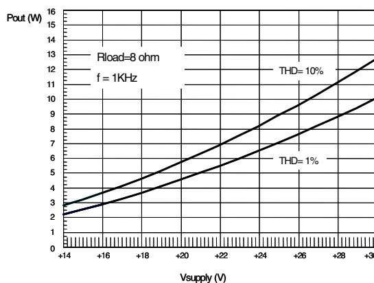
Figure 4. output power vs supply voltage (single)
