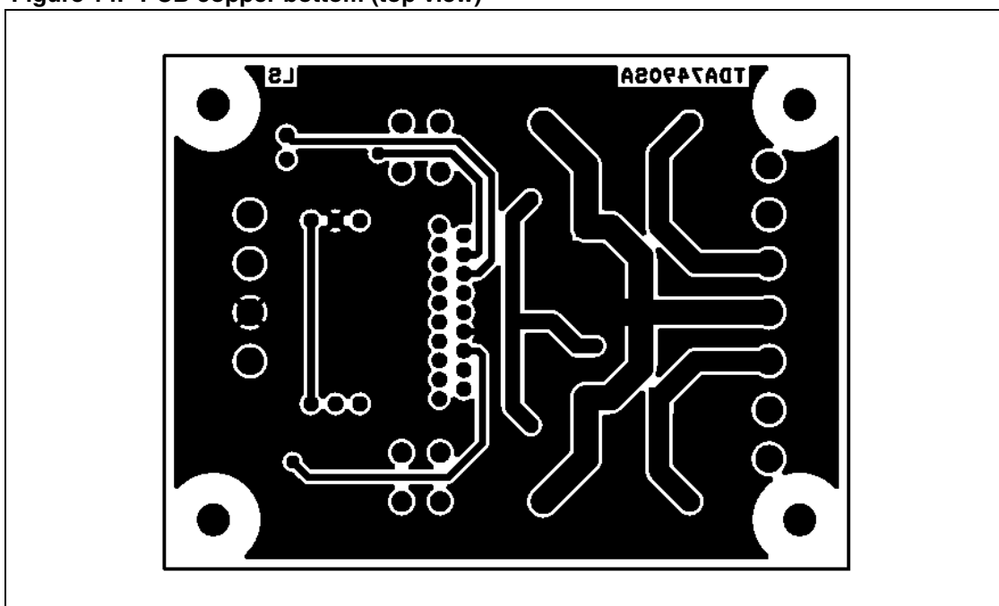
Figure 14. PCB copper bottom (top view)
