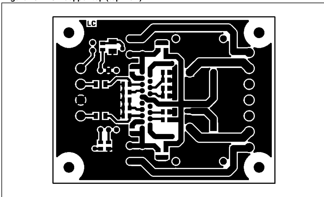
Figure 15. PCB copper top (top view)
