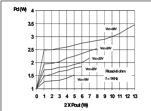
Figure 9. dissipated power vs output power
