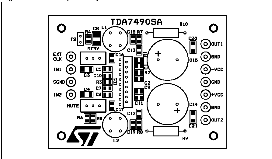
Figure 13. PCB component layout of the test circuit
