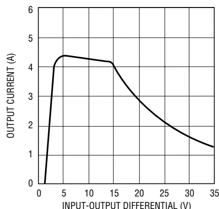
Current Limit
