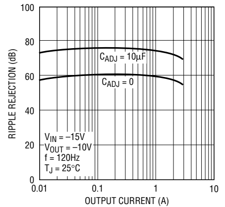
Ripple Rejection
