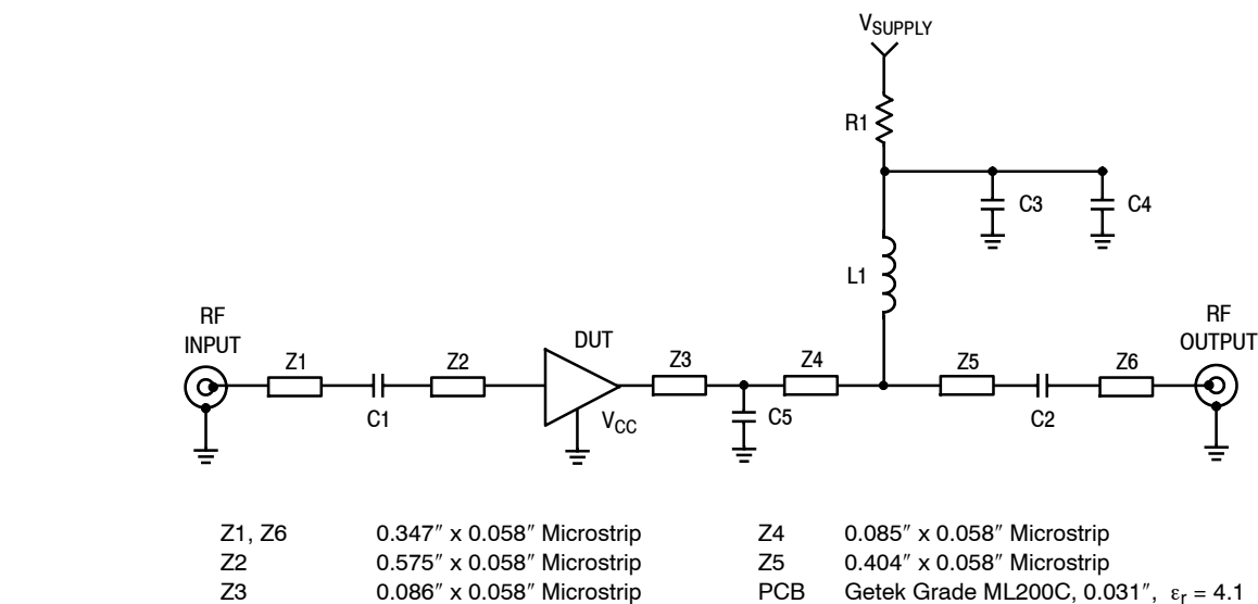
Figure 26. 50 Ohm Test Circuit Schematic
