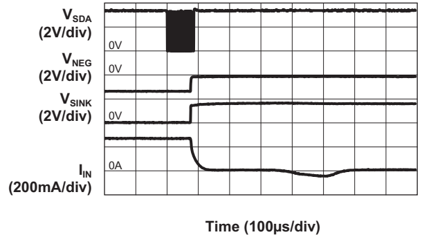
Backlight Turn OFF Characteristics, 1.5x Mode (V_{IN} = 3.6V; I_{BLX} = 19.8mA/ch)
