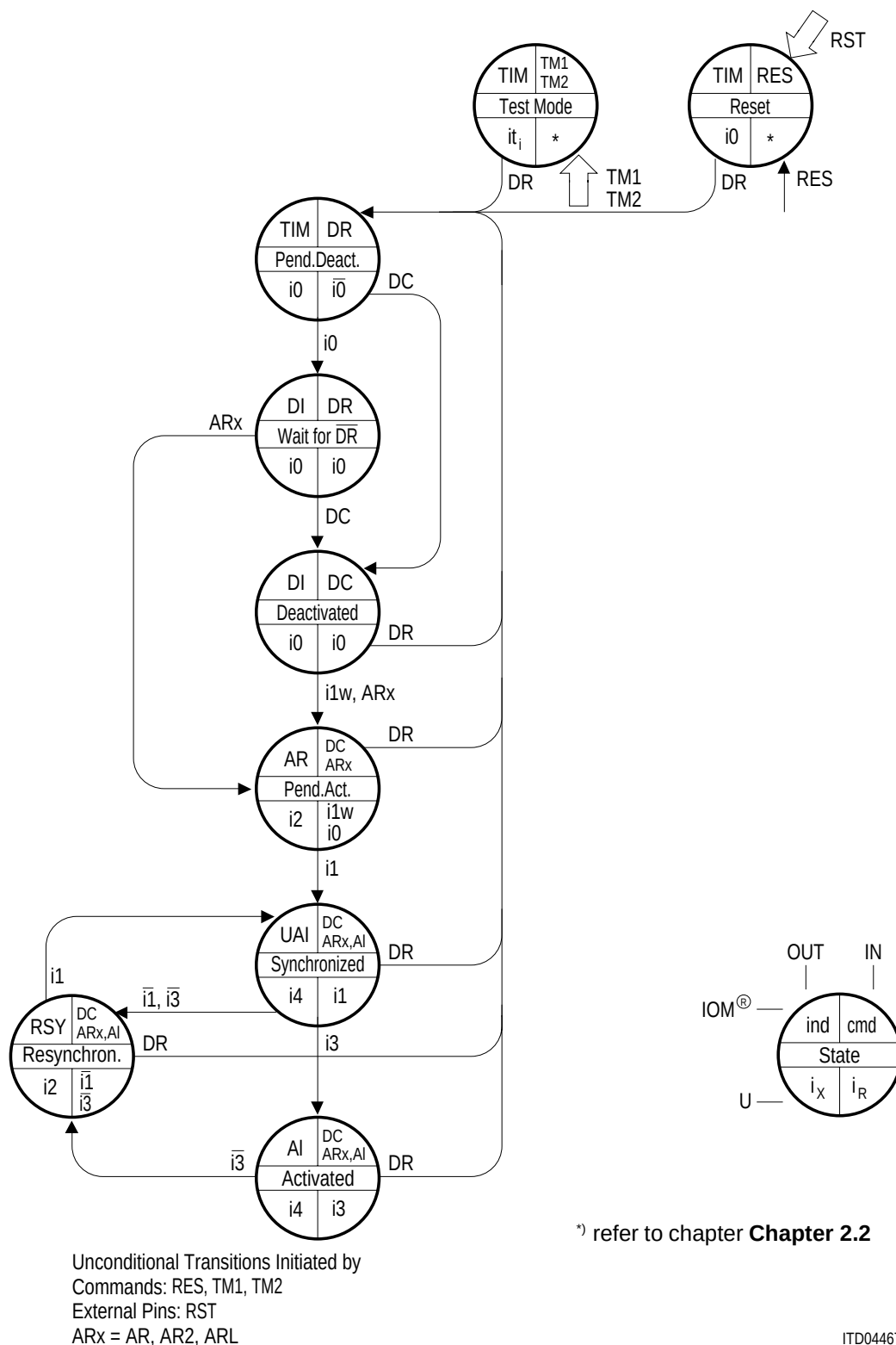
Figure 3-8 OCTAT-P State Diagram
