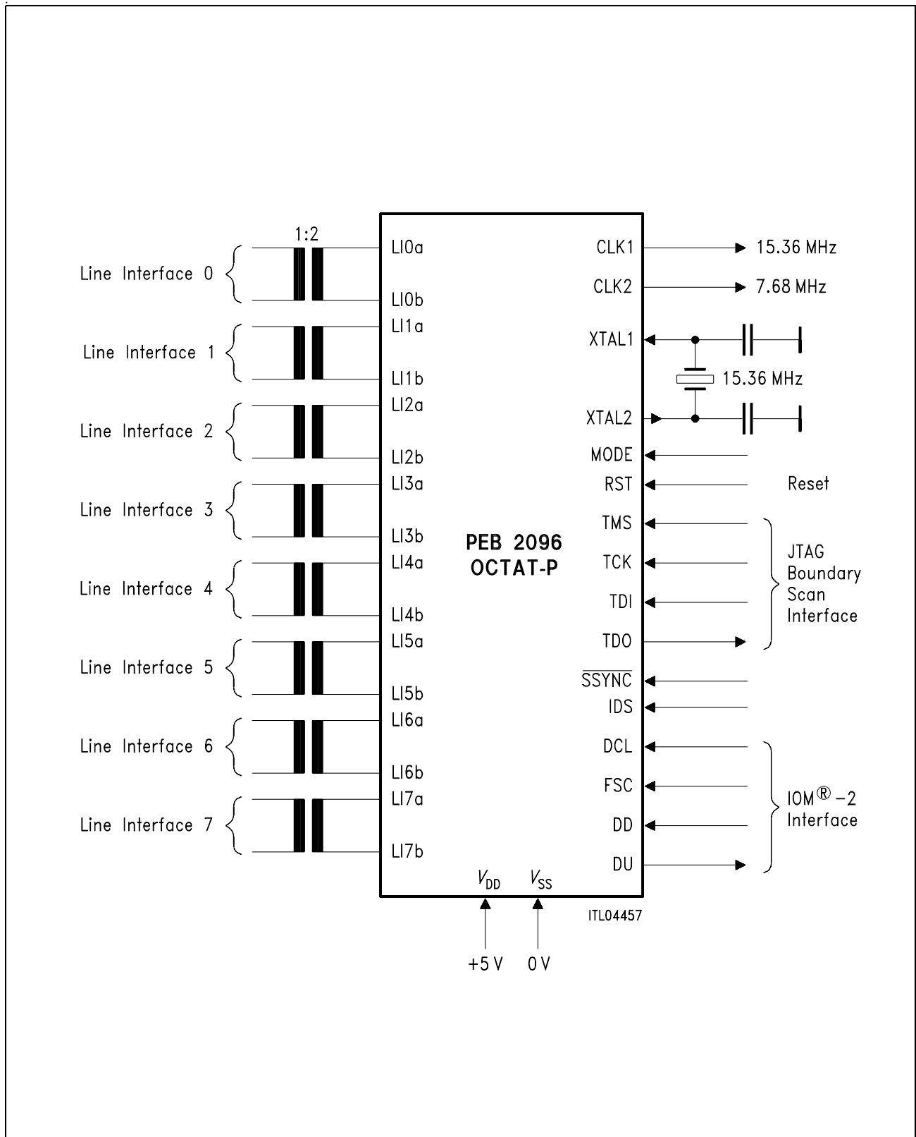
Figure 1-2 Logic Symbol
