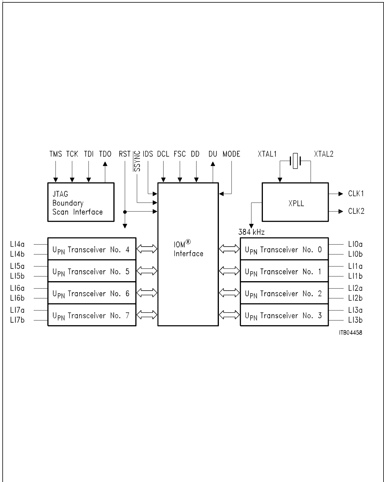
Figure 1-4 Block Diagram
