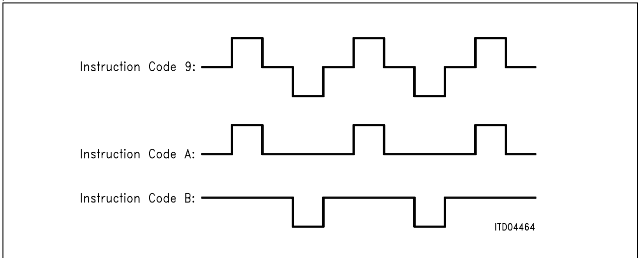
Figure 2-5 Test Pulse Wave Forms
