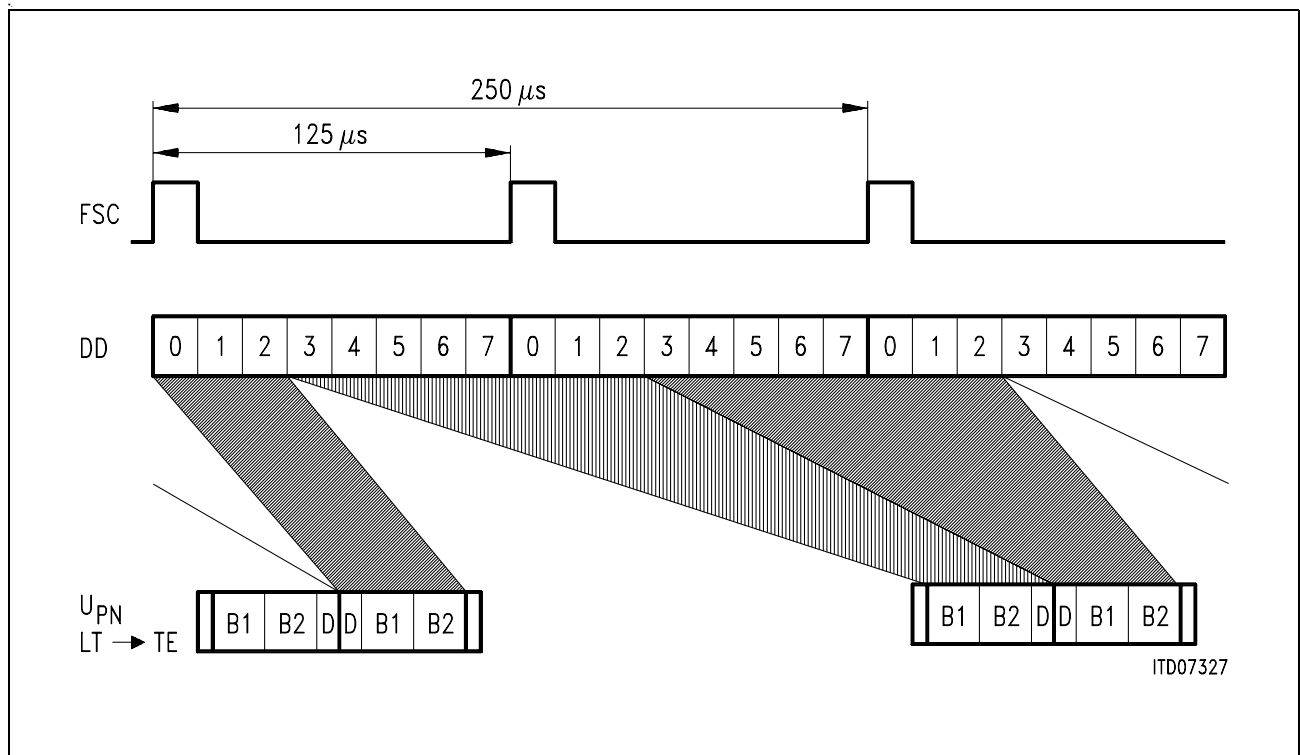
Figure 3-1 Transmit Delay of B- and D-Channels
