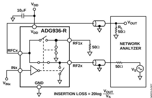
Figure 22. Insertion Loss
