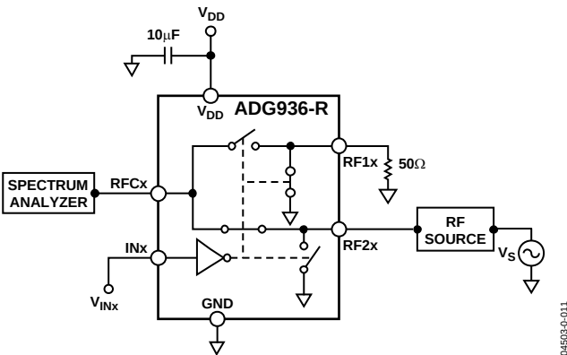
Figure 26. P_{-1dB}
