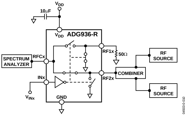
Figure 25. IP_3
