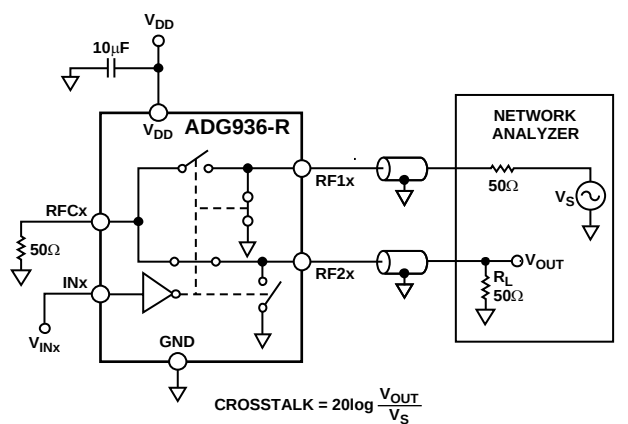
Figure 23. Crosstalk
