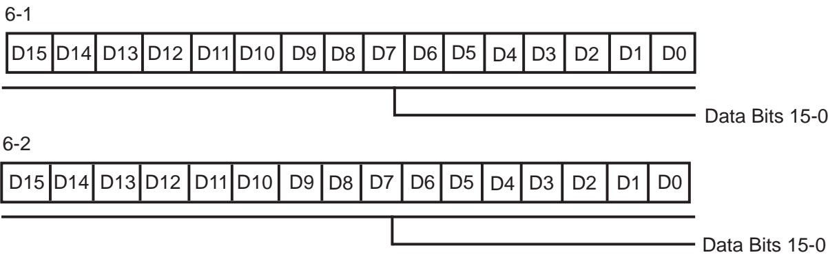
Figure 23. CODEC Interface Data Registers (Channel 1)
