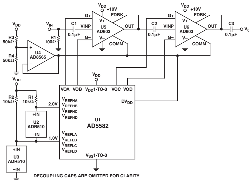
Figure 8. Programmable PGA
