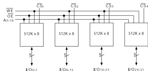
BLOCK DIAGRAM
