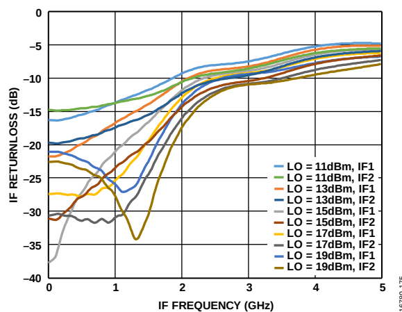
Figure 75. IF Return Loss vs. IF Frequency at Various LO Power Levels, T_A = 25^\circ\text{C} , LO = 27 GHz
