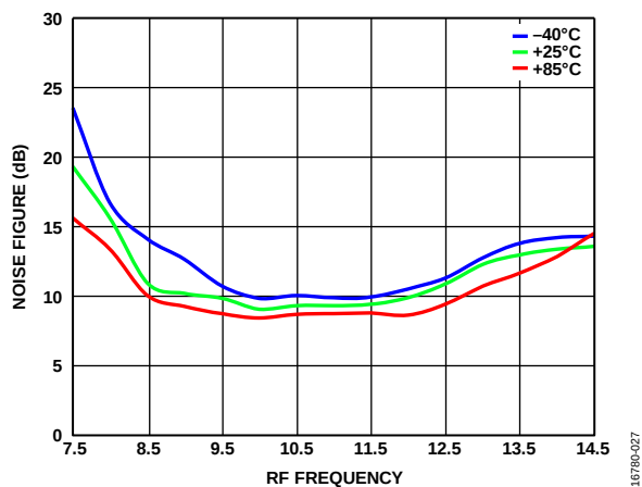
Figure 27. Noise Figure vs. RF Frequency at Various Temperatures, T_A = 25^\circ\text{C}
