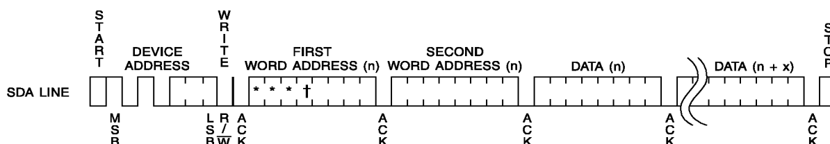
Figure 3. Page Write
