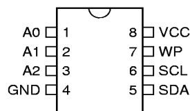
8-Pin TSSOP
