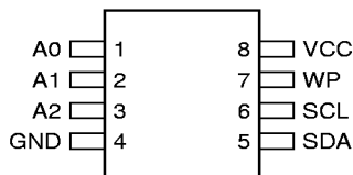
8-Pin SOIC
