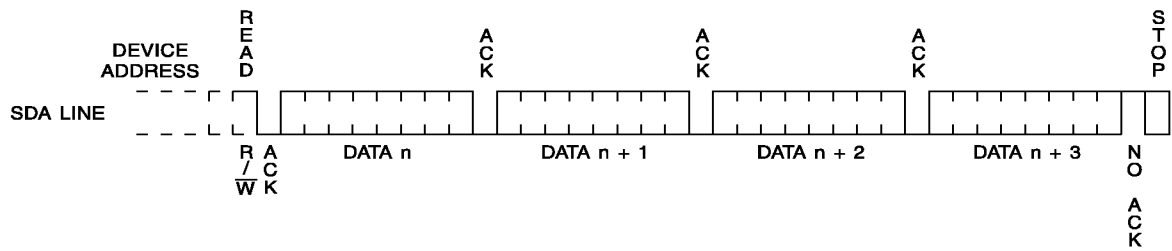
Figure 6. Sequential Read
