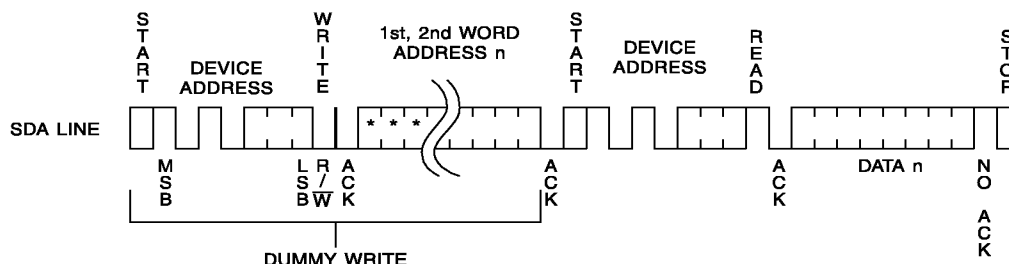
Figure 5. Random Read
