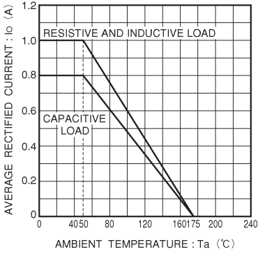
Fig.3 Derating curve
