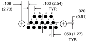
15 Contacts View X
