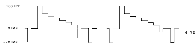
Figure xx Undershoot Limiter , programmed to -6 IRE
