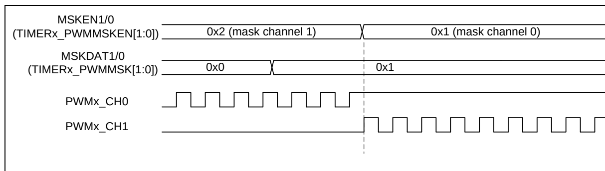
Figure 6.17-15 PWM Output Mask Control Waveform
