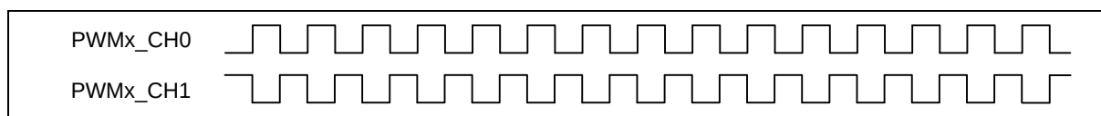
Figure 6.17-11 PWM Complementary Mode Output Waveform
