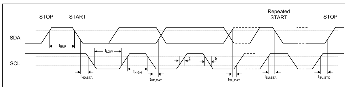
Figure 8.6-1 I 2 C Timing Diagram
