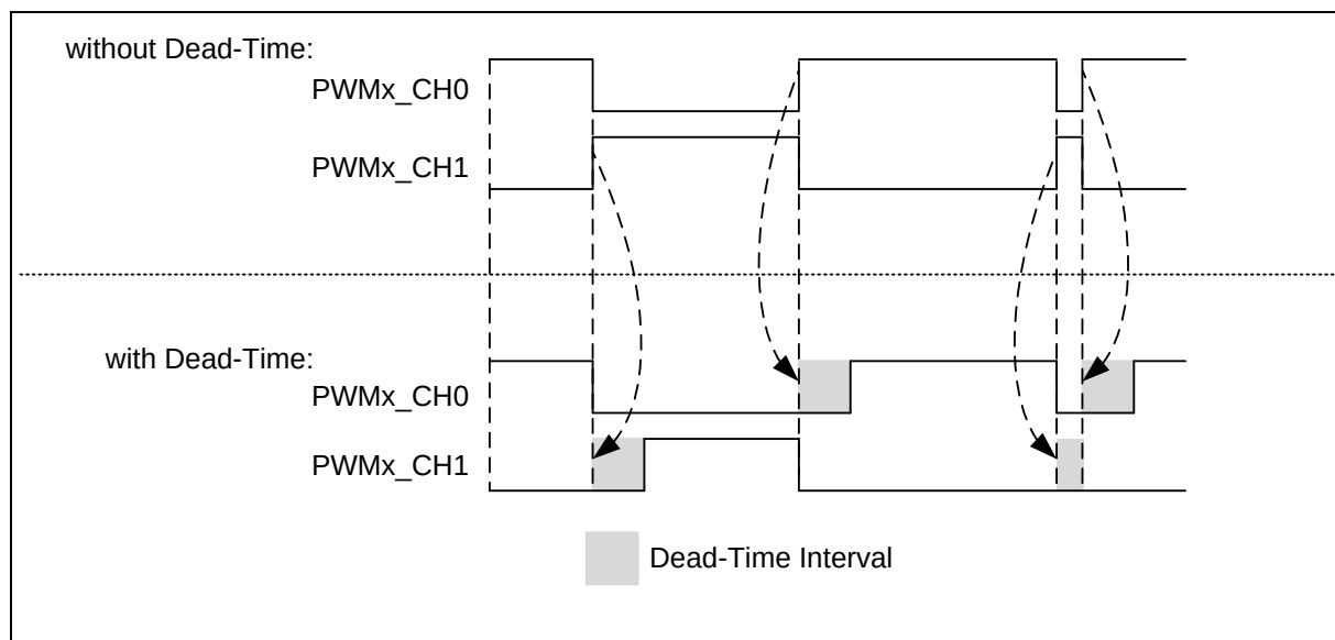
Figure 6.17-14 Dead-Time Insertion
