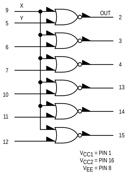
LOGIC DIAGRAM
