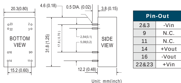
▲ SCW05 1.25" x 0.80" x 0.48"
