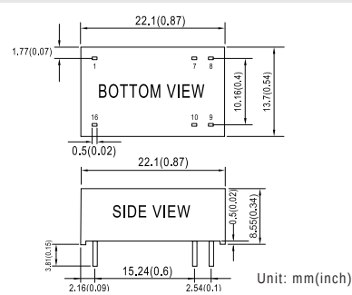
▲ DLC03 0.87" x 0.54" x 0.34"
