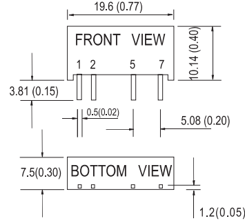
▲ SPU03 0.77" x 0.30" x 0.40"
