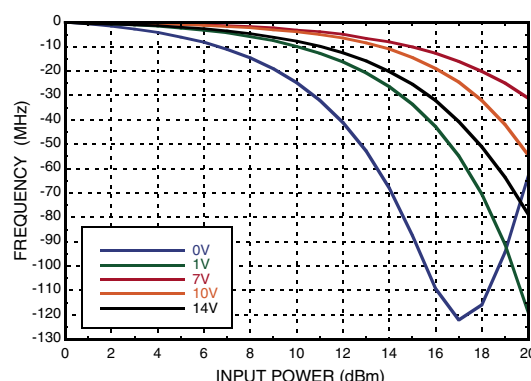
F_{center} vs. Input Power V_{fctl} = V_{nctl}
