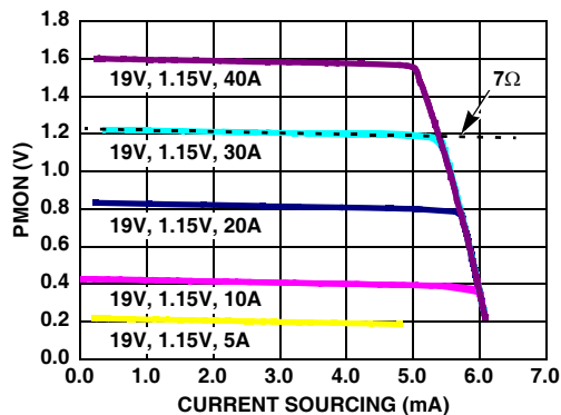
FIGURE 35. POWER MONITOR CURRENT SOURCING CAPABILITY
