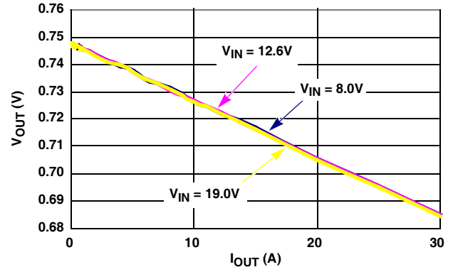
FIGURE 12. DEEPER SLEEP MODE LOAD LINE, 2 PHASE, DCM OPERATION, PSi# = LOW, VID = 0.75V
