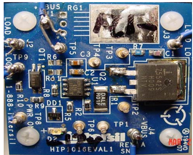
FIGURE 7. ISL6116 EVAL BOARD PICTURE
