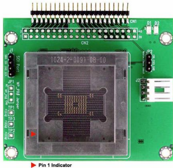
Figure 2: NANDrive Socket Board, 44-pin Connector
