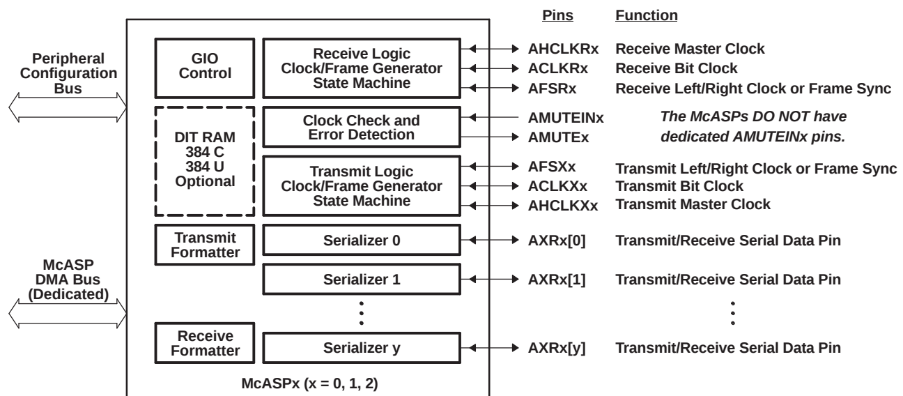
Figure 5-33. McASP Block Diagram
