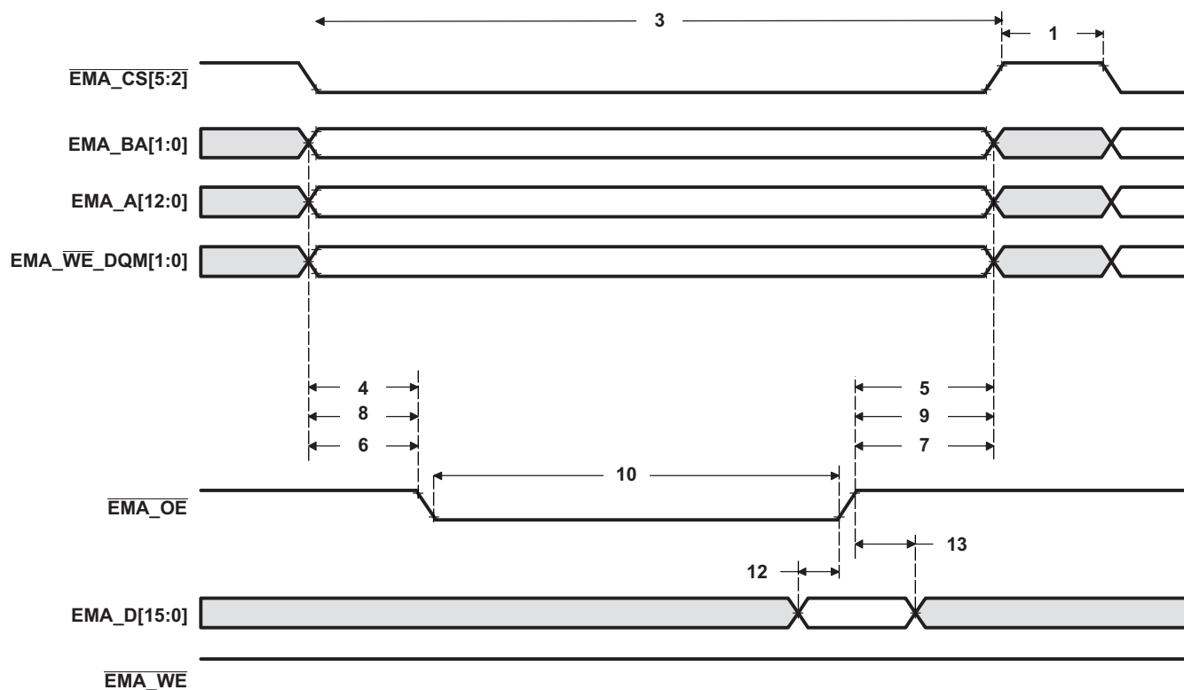
Figure 5-16. Asynchronous Memory Read Timing for EMIFA
