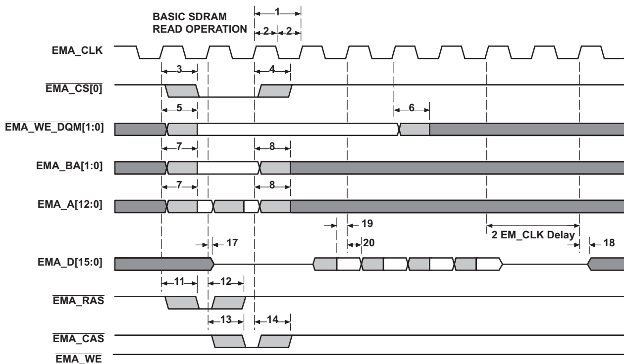
Figure 5-15. EMIFA Basic SDRAM Read Operation
