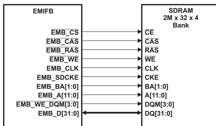
Figure 5-22. EMIFB to 2M × 32 × 4 bank SDRAM Interface
