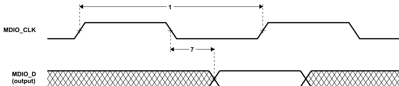
Figure 5-32. MDIO Output Timing
