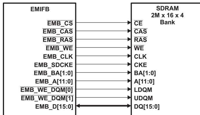
Figure 5-21. EMIFB to 2M × 16 × 4 bank SDRAM Interface
