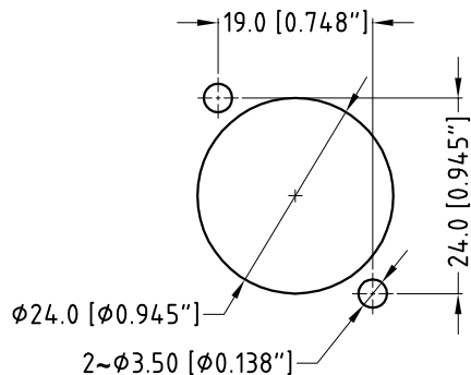
PANEL CUTOUT
