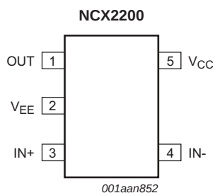
Fig 2. Pin configuration SOT353-1
