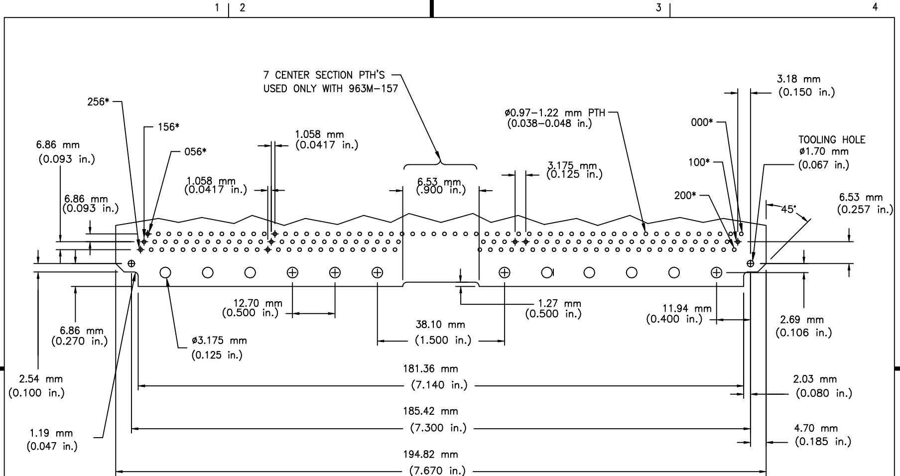
RECOMMENDED PC BOARD HOLE PATTERN (COMPONENT SIDE)
