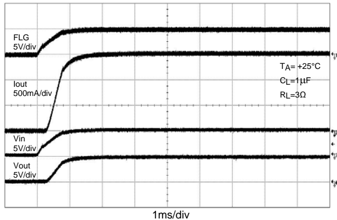
Device Enabled
