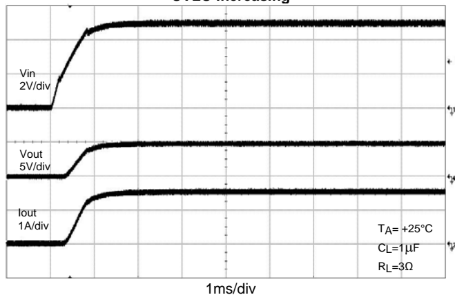
UVLO Increasing
