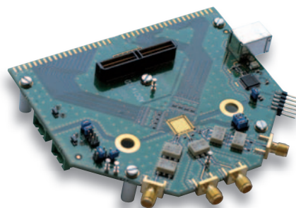
LVDS/DDR digital outputs (F2/DB)
