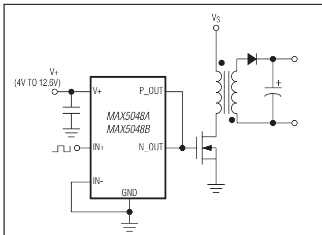
Figure 3. Noninverting Application
