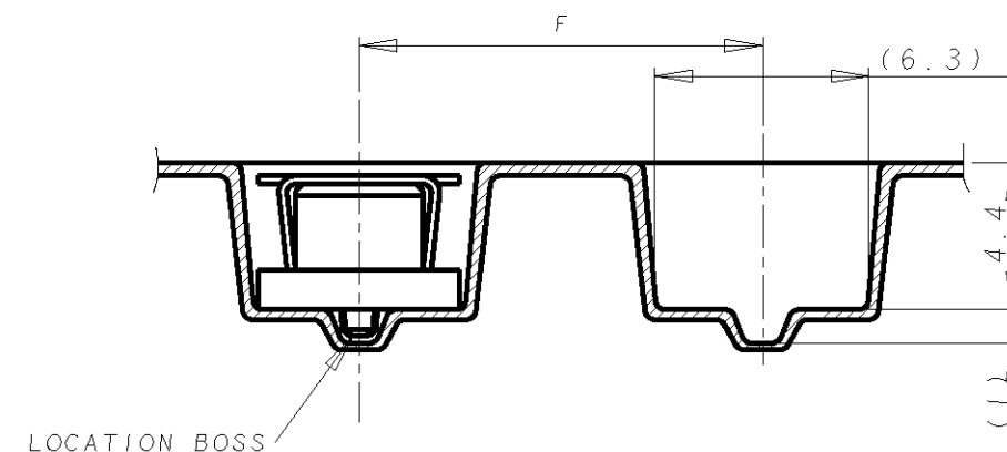
DETAIL A (SCALE 4-1)
