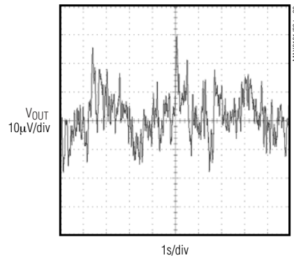
MAX6165 NOISE
