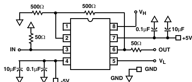
FIGURE 2C. SCHEMATIC
