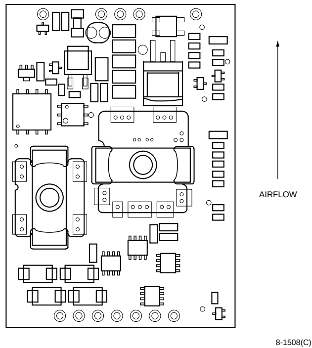
Figure 19. Worst Orientation (Top View)
