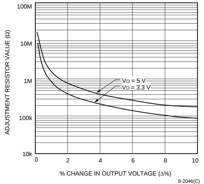
Figure 16. Resistor Selection for Increased Output Voltage
