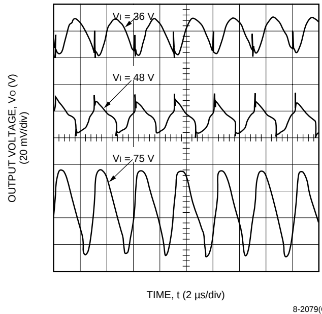
Figure 6. Typical HW100A1 Output Ripple Voltage at Room Temperature and I_o = I_{o,max}
