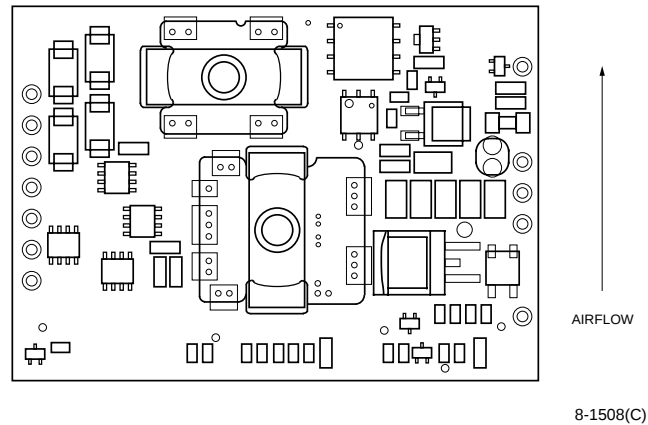
Figure 18. Best Orientation (Top View)
