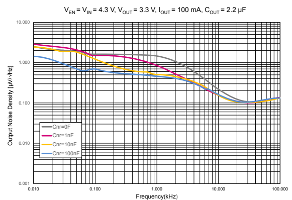
Figure 23. Output noise spectrum vs. C_{NR}
