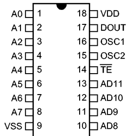
HT12E -18 DIP
