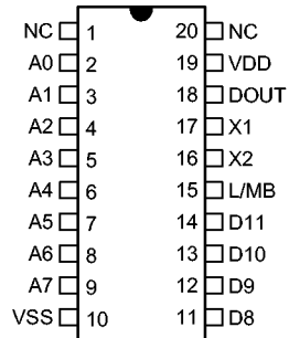
HT12A -20 SOP
