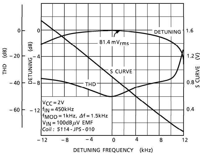
IF DETUNING CHARACTERISTICS
