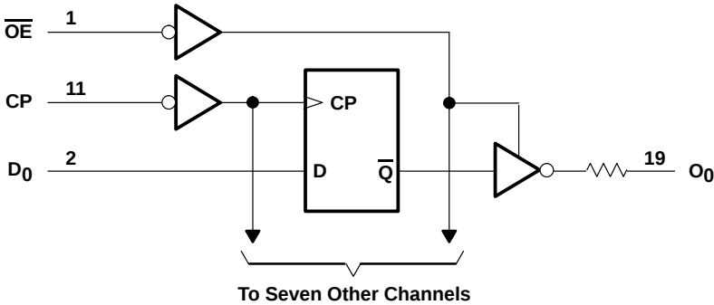
logic diagram (positive logic)
