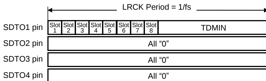
Figure 57. Slot Assign in PCM Mode
