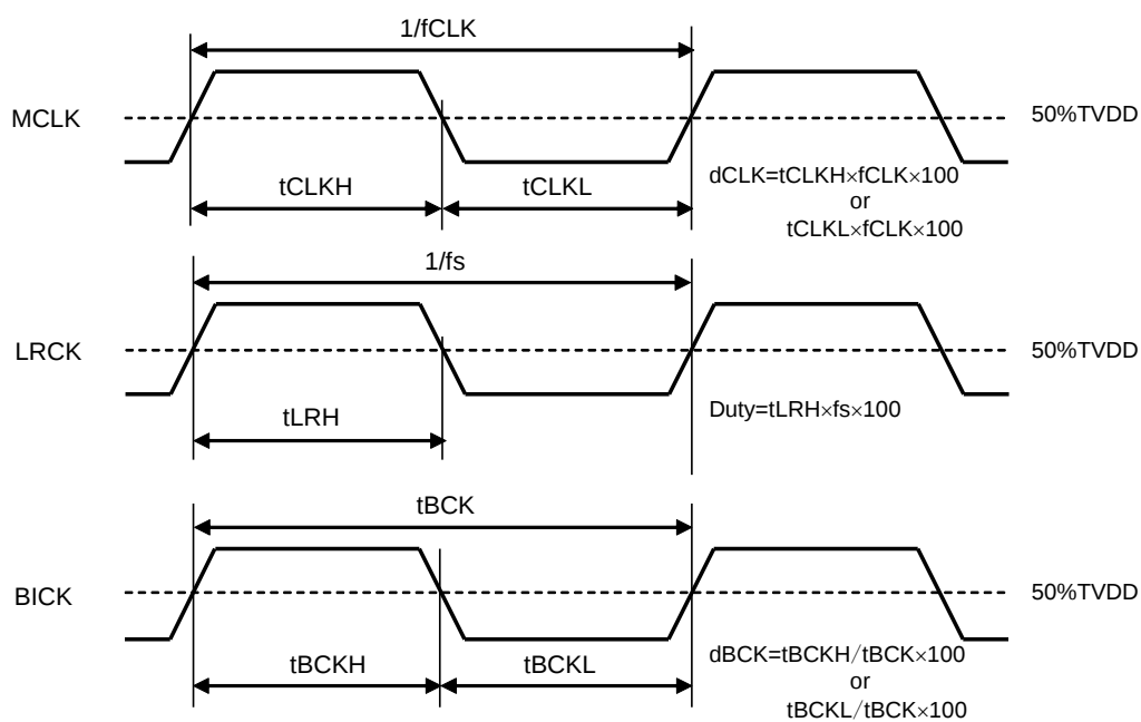
Figure 18. Clock Timing (Master Mode)
