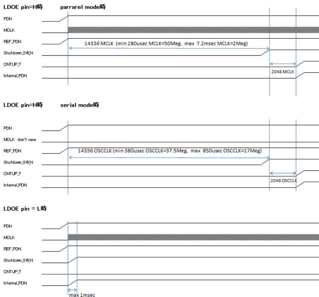
Figure 60. Internal PDN Release Sequence
