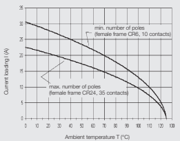
ConCept module CM-5 Conductor H07V-K 4.0 mm 2
