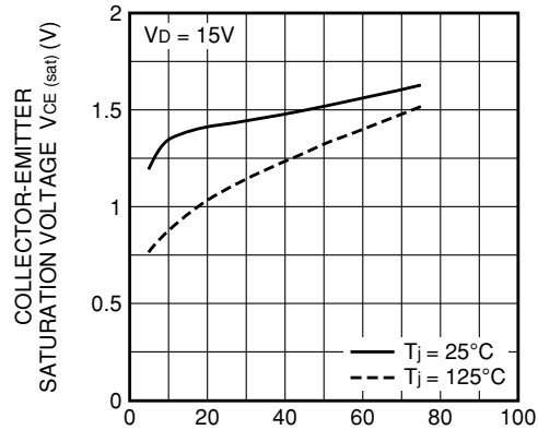
COLLECTOR-EMITTER SATURATION VOLTAGE (VS. I_c ) CHARACTERISTICS (TYPICAL)
