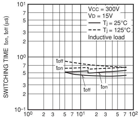
SWITCHING TIME CHARACTERISTICS (TYPICAL)
