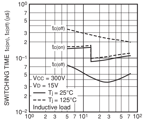
SWITCHING TIME CHARACTERISTICS (TYPICAL)
