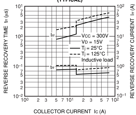
FWDi REVERSE RECOVERY CHARACTERISTICS (TYPICAL)
