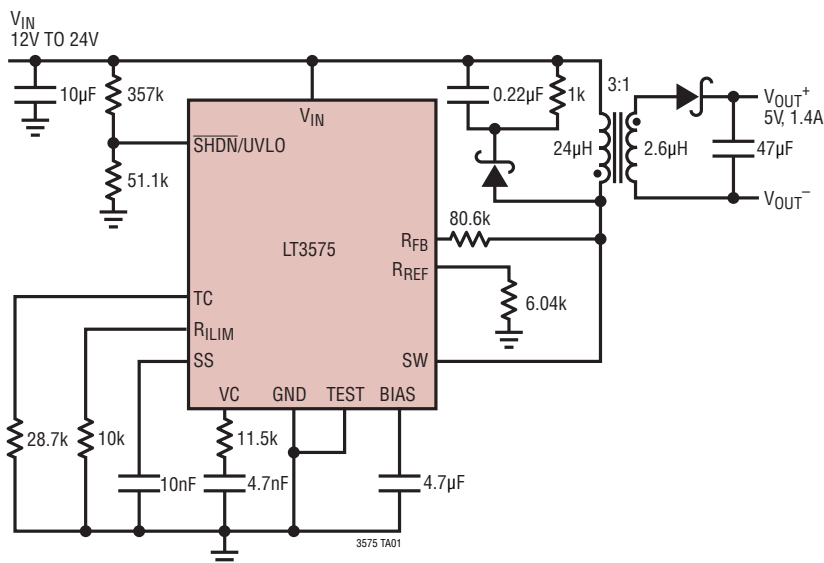
5V Isolated Flyback Converter
