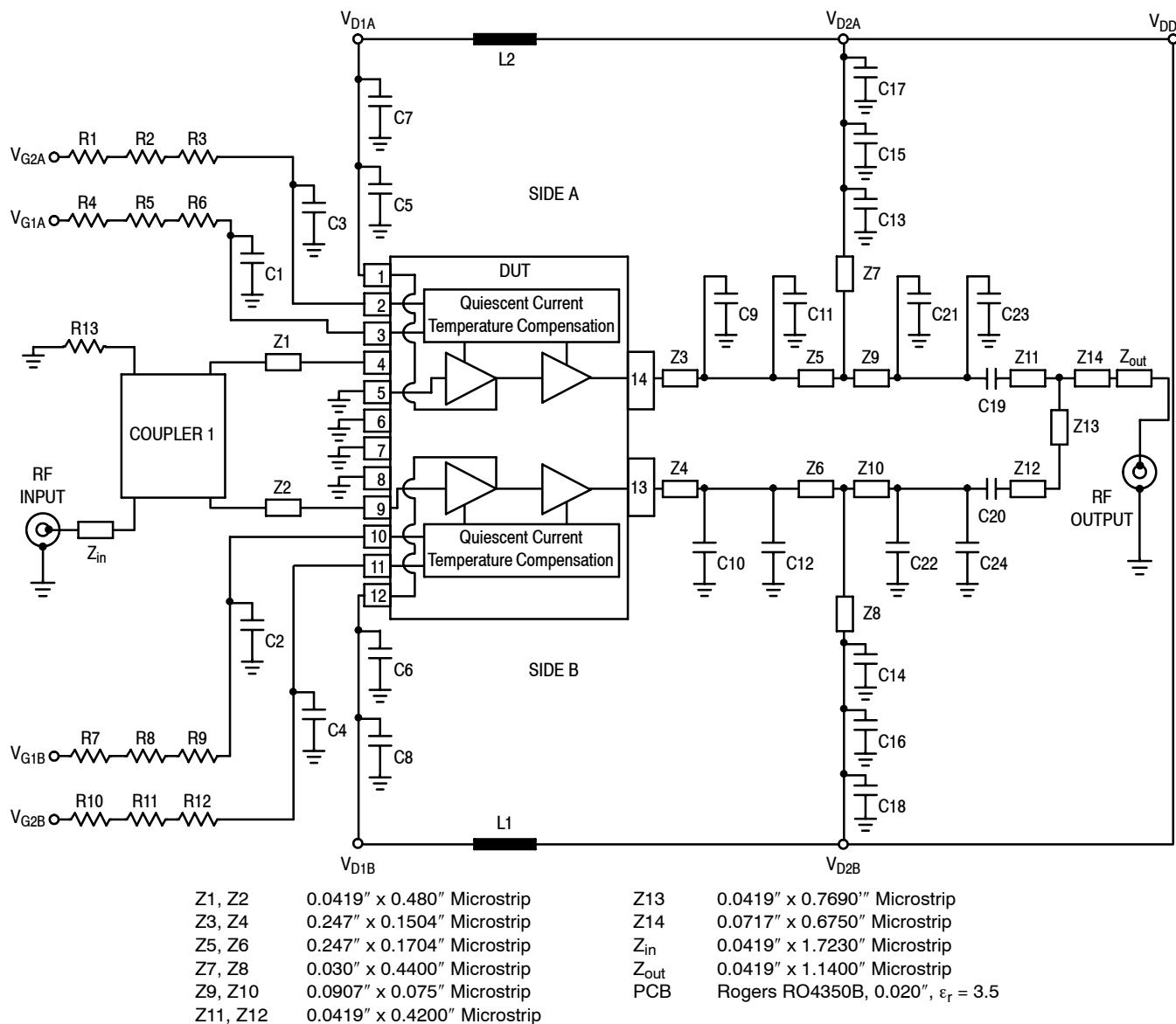
Figure 3. MD7IC2755NR1(GNR1) Test Circuit Schematic
