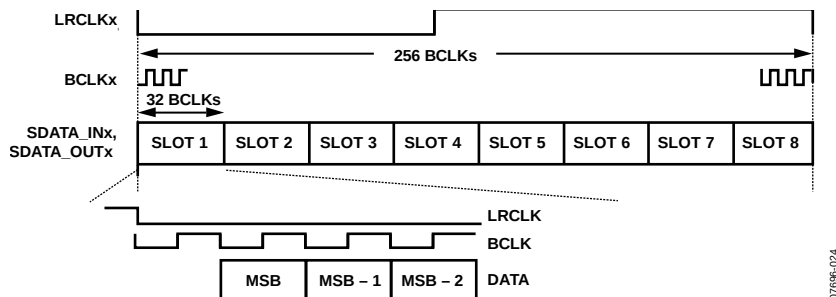
Figure 25. TDM Mode
