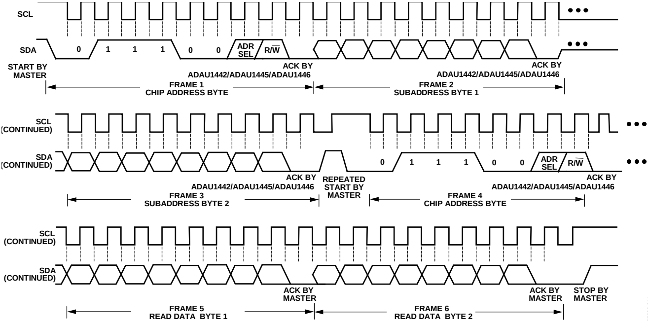
Figure 14. I 2 C Read Clocking
